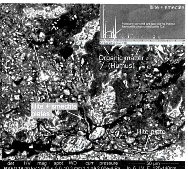
Fig. 6. A suspected bentonite (Northern Lithuania, Joniškėlis)
