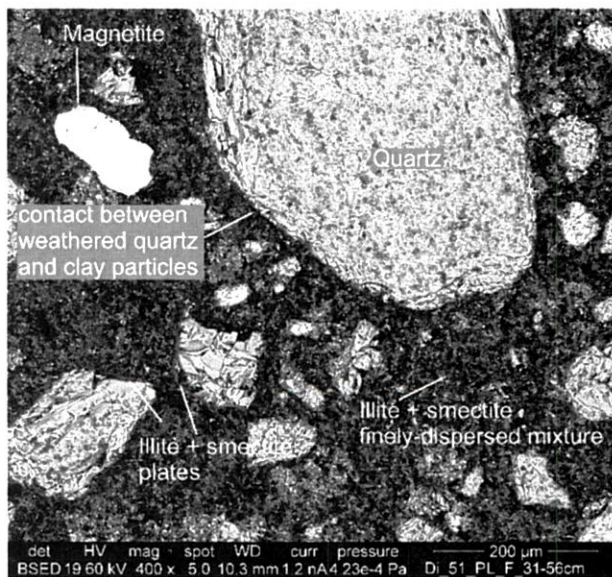
Fig. 1c. Weathered quartz in the soil of the Middle Pleistocene deposits (Southeast Lithuania, Dieveniškės)
