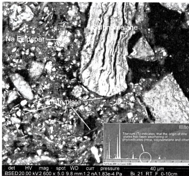
Fig. 4a. Clay minerals formed in weathered phyllosilicates (mica, stilpnomelane and others) in the soil of the Upper Pleistocene deposits (Western Lithuania, Bijotai)
