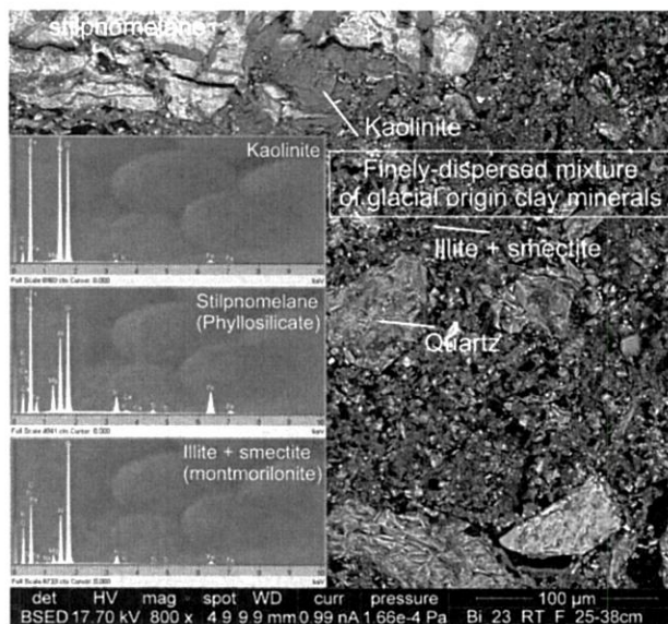
Fig. 2. Clay minerals of presumably glacial origin in the soil of the Upper Pleistocene deposits
