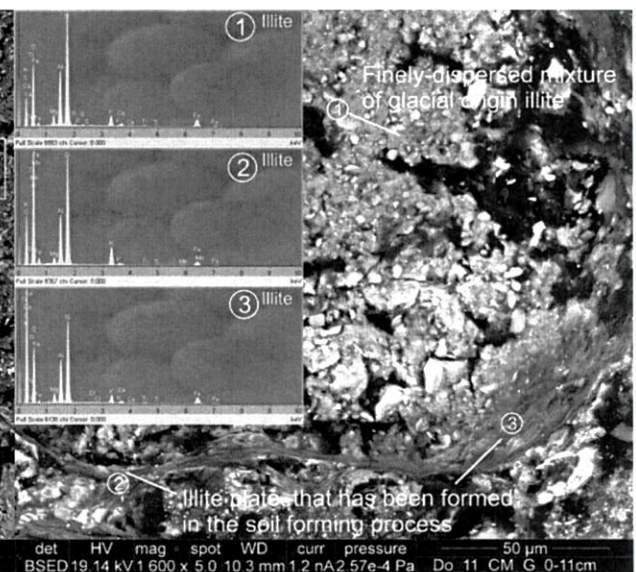
Fig. 3. Clay minerals of presumably pedogenic origin in the soil of the Upper Pleistocene deposits
