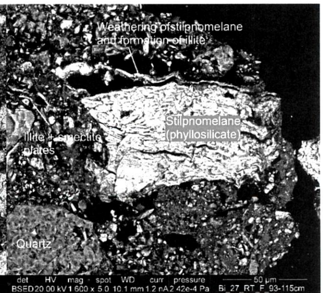
Fig. 1d. Weathered phyllosilicate (stilpnomelane) in the soil of the Upper Pleistocene deposits (Western Lithuania, Bijotai)
