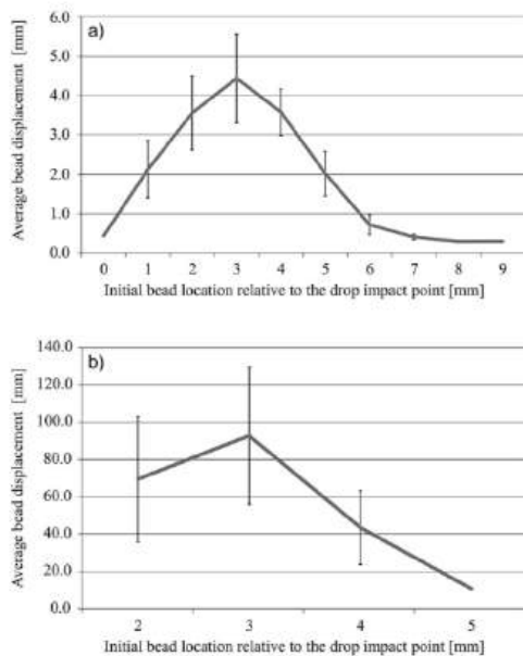
Fig. 8. Average displacements of beads from the saturated beds depending on the initial position, for: (a) beads displaced in the deformation, (b) ejected beads. The vertical lines denote standard deviations.
