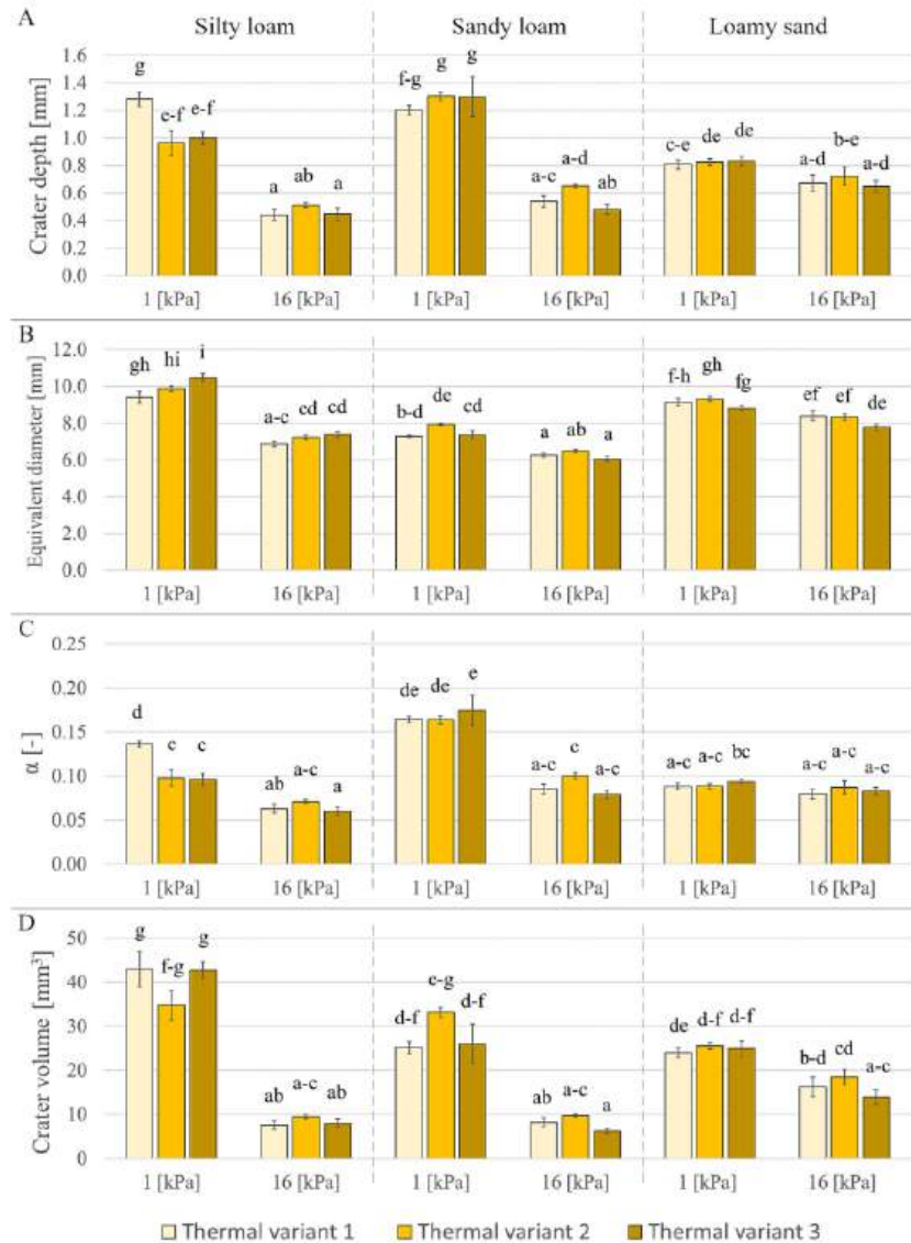
Fig. 5. Average values of the determined quantities: A – depth of craters; B – equivalent diameter; C – depth to diameter ratio; D – volume of craters. Bars indicate standard errors. The results of Tukey's post-hoc test are shown by the letters above the bars. The statistical test for each quantity involved comparing all variants with each other – the same letters indicate no statistically significant differences within individual quantities. Variant results belonging to three or more groups have been marked with ranges, for example a-c.
