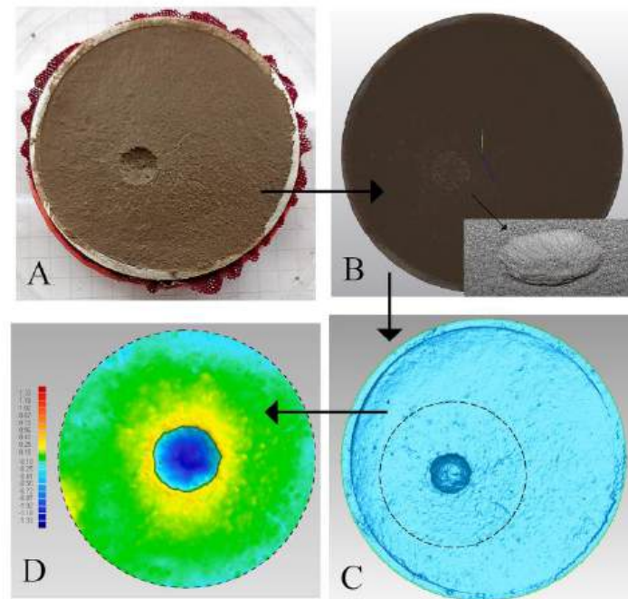
Fig. 4. Steps in processing data obtained with the Smarttech3D scanner during crater morphology measurements: A – soil sample with a crater after a drop impact; B – calibrated point clouds with detail; C – triangle mesh of the crater; D – height map of the area around the crater marked by the circle on the triangle grid (crater depth measurement).
