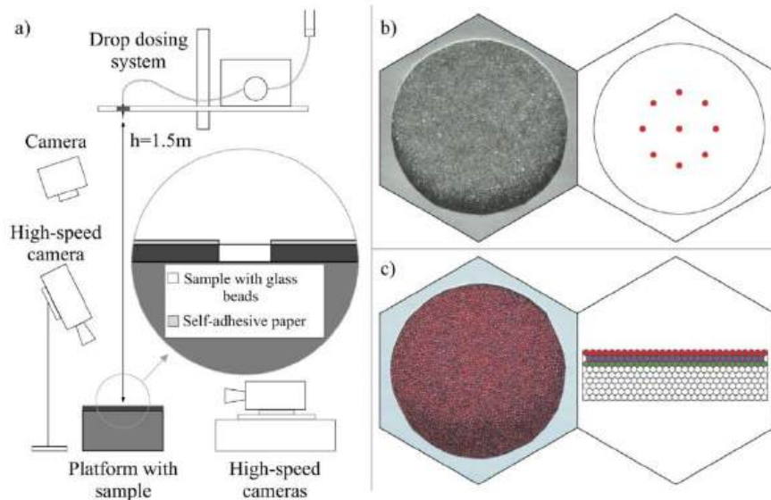
Fig. 1. Experimental set-up: (a) diagram of the measuring stand and (b) example of bed containing the pattern (photo plus scheme), (c) example of bed with layers of beads of the same colour (photo plus scheme). (For interpretation of the references to colour in this figure legend, the reader is referred to the web version of this article.)
