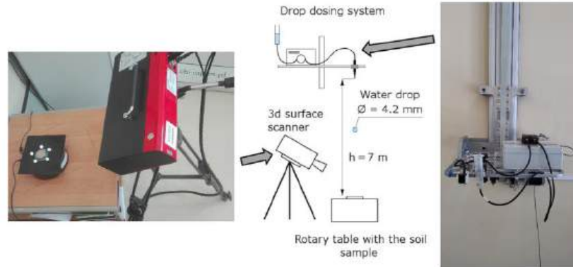
Fig. 2. Diagram of the measuring stand with a picture of the surface scanner (left) and the drop dispensing system (right).
