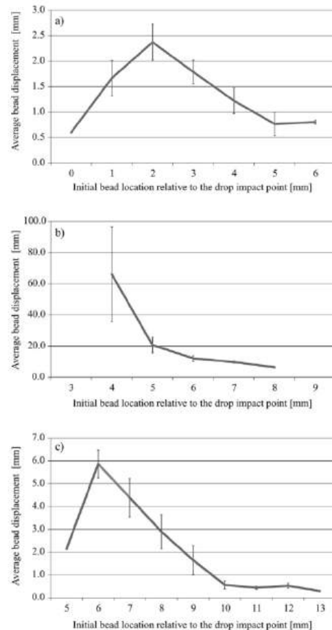
Fig. 6. Average displacements of beads from the dry bed depending on the initial position, for: (a) beads displaced in the wet area, (b) ejected beads, and (c) beads placed on the rim. The vertical lines denote standard deviations.
