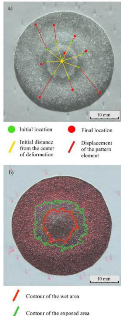
Fig. 2. Analysis of samples in the GIMP program: (a) bed containing the pattern, (b) bed with layers of beads of the same colour. (For interpretation of the references to colour in this figure legend, the reader is referred to the web version of this article.)
