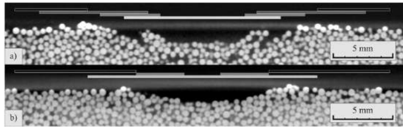
Fig. 11. Examples of deformation cross sections prepared using microtomography: (a) dry bed, (b) saturated bed. The lines above the cross sections represent the areas of occurrence of the different types of bead displacements shown in Fig. 5, Fig. 6, Fig. 7 and Fig. 8.
