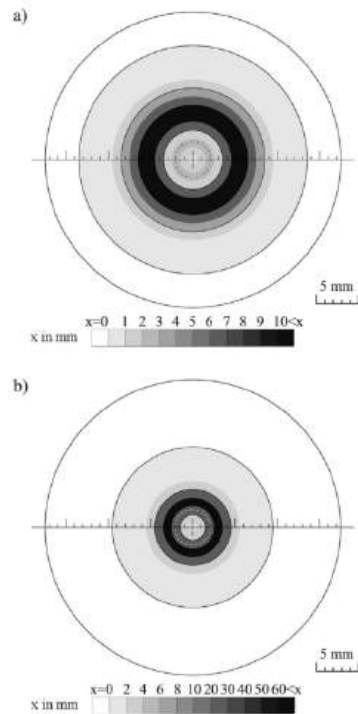
Fig. 5. Average distances over which the beads were displaced depending on their initial position for: (a) the dry bed, (b) the saturated bed. The outer circle in the drawing shows the size of the aluminium rings in which the beds were prepared. X represents the average displacement of beads in millimetres, also indicated by shades of grey.
