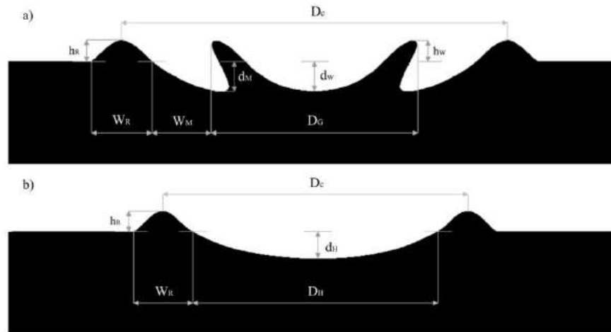
Fig. 3. Diagram of deformation with parameters measured by the microtomograph for (a) the dry sample and (b) the saturated sample, where h_R is the rim height, h_W is the wetted area height, d_M is the moat depth, d_W is the wetted area depth, d_H is the hole depth, W_R is the rim width, W_M is the moat width, D_G is the diameter of the wetted area, D_H is the diameter of the hole, and D_C is the diameter of the crater.
