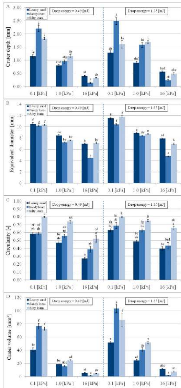
Fig. 2. Average values of the determined quantities: A – depth of craters; B – equivalent diameter; C – circularity; D – volume of craters. Bars indicate standard errors. The results of Tukey's post-hoc test are shown by the letters above the bars.
