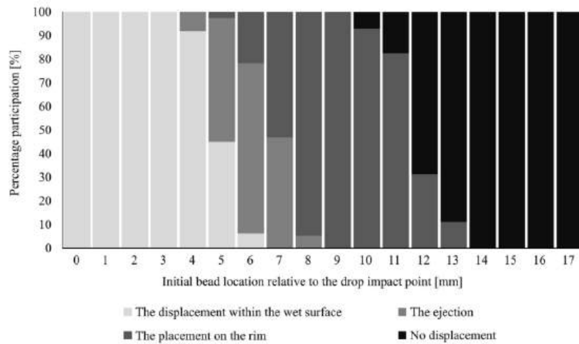
Fig. 7. Percentage of beads with different types of displacement in areas defined based on their initial location. Results for the dry beds.
