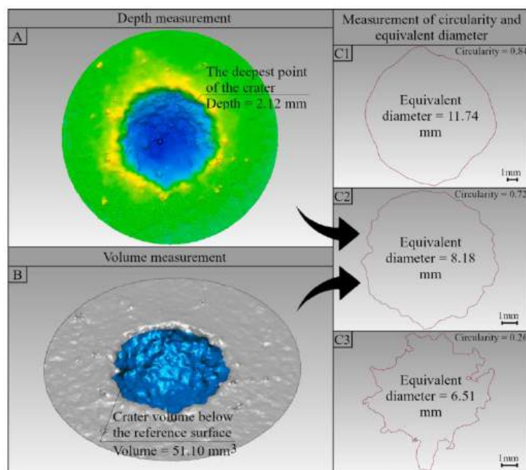
Fig. 1. Examples of analysed crater quantities: A – depth of crater; B – volume of crater; C – sample cross-sections with different circularity: C1 – silty loam at a pressure head equal to 0.1 kPa and the drop falling from 7 m; C2 – sandy loam at a pressure head equal to 1 kPa and the drop falling from 7 m; C3 – loamy sand at a pressure head equal to 16 kPa and the drop falling from 1.5 m.
