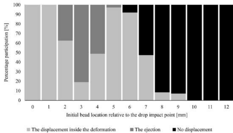
Fig. 9. Percentage of beads with different types of displacement in areas defined based on their initial location. Results for the saturated beds.
